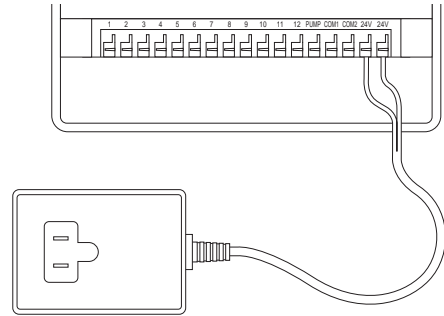
FIGURE 17: Connecting Transformer
